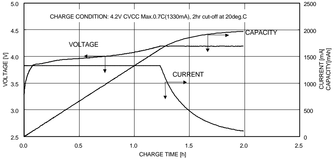
CHARGE CHARACTERISTICS OF CGR18650A
