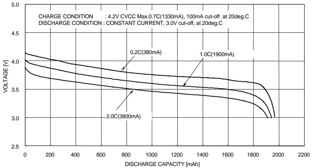
DISCHARGE CHARACTERISTICS OF CGR18650A
