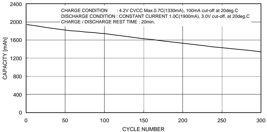
CYCLE LIFE CHARACTERISTICS OF CGR18650A
