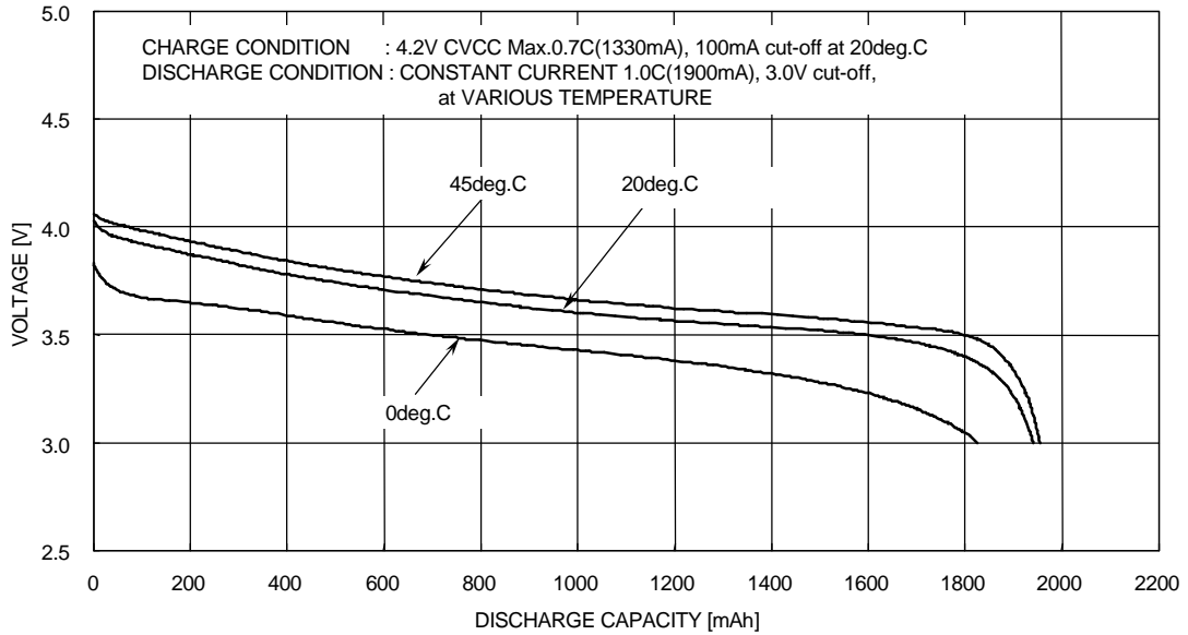
DISCHARGE CHARACTERISTICS OF CGR18650A
